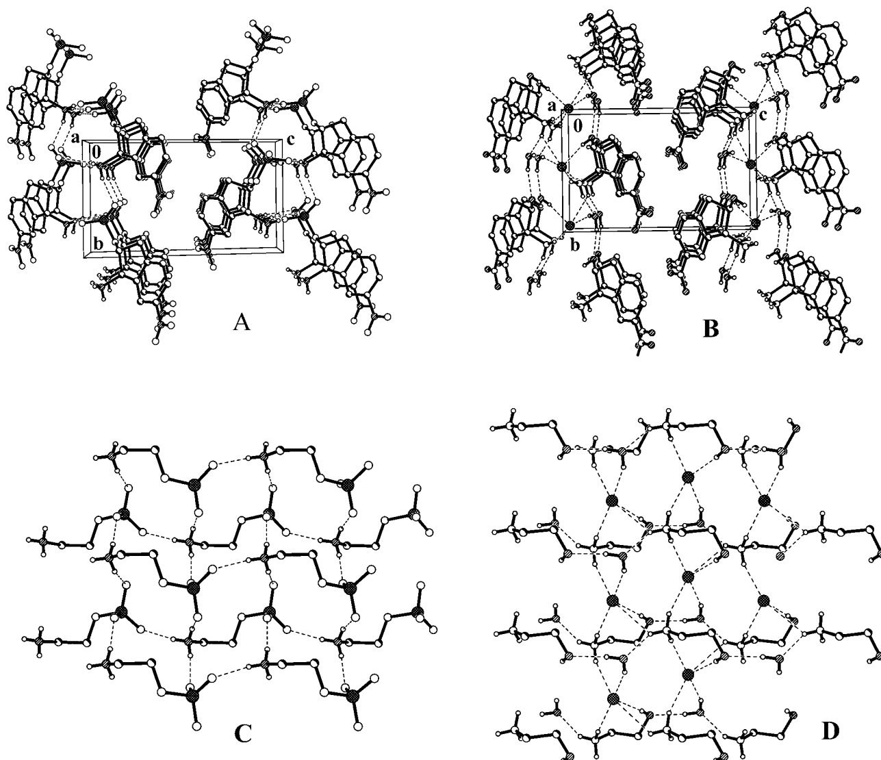
Figure 2. Crystal packing of (1 R ,2 R )- trans -1-amino-6-nitroindan-2-ol hydrochloride monohydrate [(1 R ,2 R )- 1 ·HCl·H 2 O] (A), of sulfuric acid mono-[(1 R ,2 R )- trans -1-amino-6-nitroindan-2-yl] ester [(1 R ,2 R )- 10 ] (B) and detailed scheme of the hydrogen bonding motifs (C and D, respectively) in the crystal.
