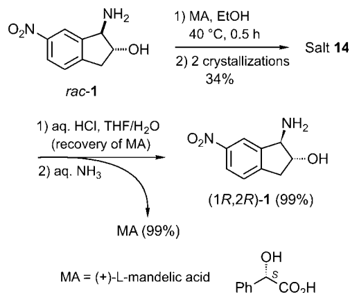
Scheme 4. Preparation of (1 R ,2 R )- trans -1-amino-6-nitroindan-2-ol [(1 R ,2 R )- 1 ] by deracemization of rac - 1 with (+)-( S )-L-mandelic acid (MA).
