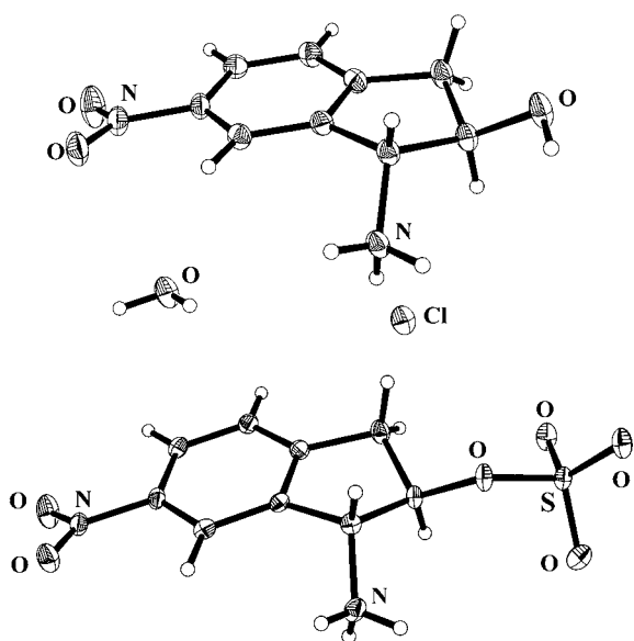
Figure 1. Molecular structures of (1 R ,2 R )- trans -1-amino-6-nitroindan-2-ol hydrochloride monohydrate [(1 R ,2 R )- 1 ·HCl·H 2 O] (top) and of sulfuric acid mono-[(1 R ,2 R )- trans -1-amino-6-nitroindan-2-yl] ester [(1 R ,2 R )- 10 ] (bottom) in the crystal. [26]
