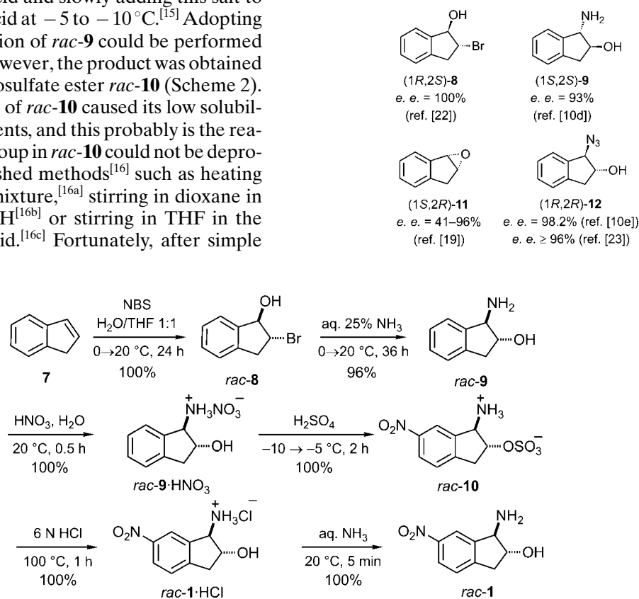
Scheme 2. Synthesis of racemic (1 R *,2 R *)- trans -1-amino-6-nitroindan-2-ol ( rac - 1 ) by direct nitration of 1-aminoindan-2-ol rac - 9 .
