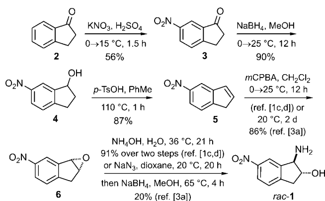
Scheme 1. Known preparations of racemic (1 R *,2 R *)- trans -1-amino-6-nitroindan-2-ol ( rac - 1 ). [1c, d, 3a, 8]
