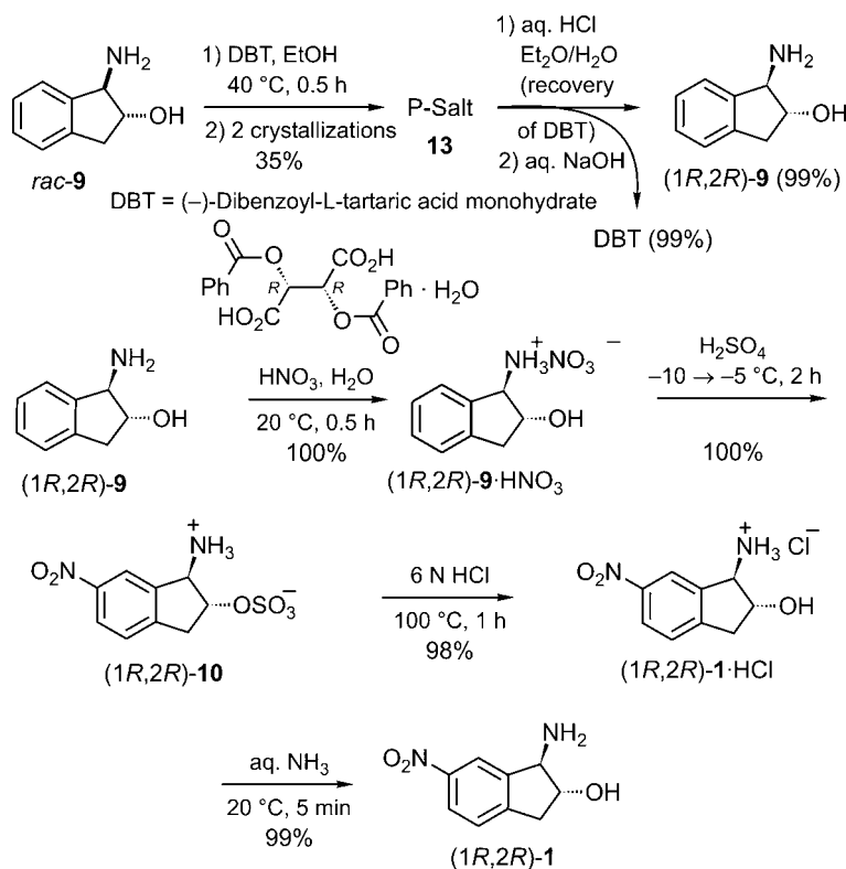
Scheme 3. Deracemization of rac - 9 with (–)-dibenzoyl-L-tartaric acid (DBT) and conversion of (1 R ,2 R )- 9 into (1 R ,2 R )- 1 by nitration.
